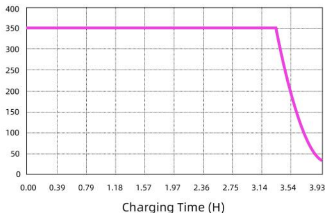
Charging Current Diagram By USB-C (Input Power 5V 0.5A)
